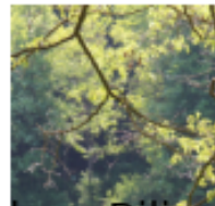
Edges Bilinear
