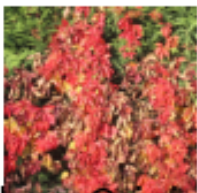
Edges Original
