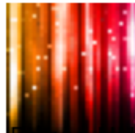
Edges NN
