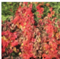
Edges Bilinear
