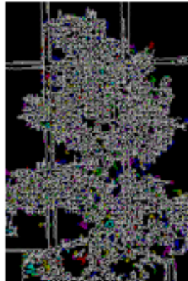
Edges NN
