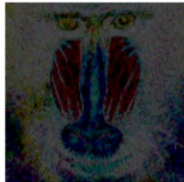
Edges NN
