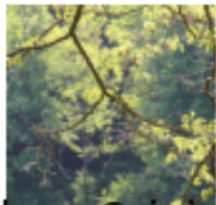
Edges Original
