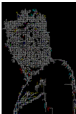
Edges NN
