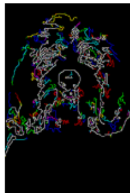
Edges Bilinear
