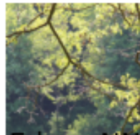
Edges NN
